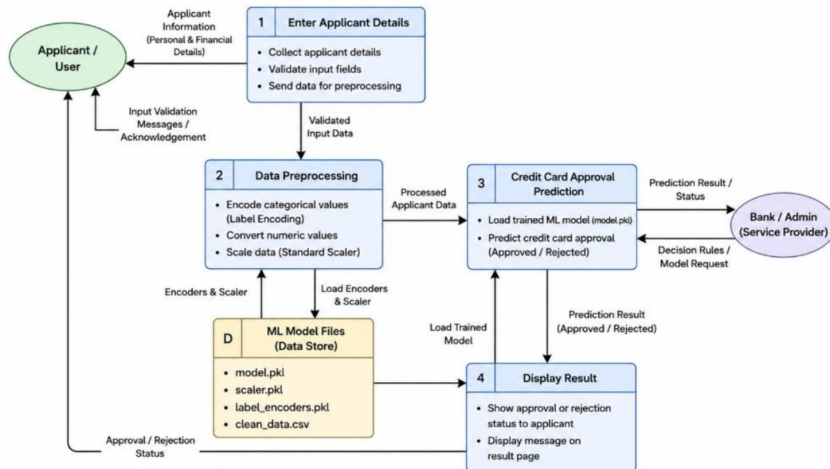
Data Flow Diagram – Credit Card Approval Prediction
